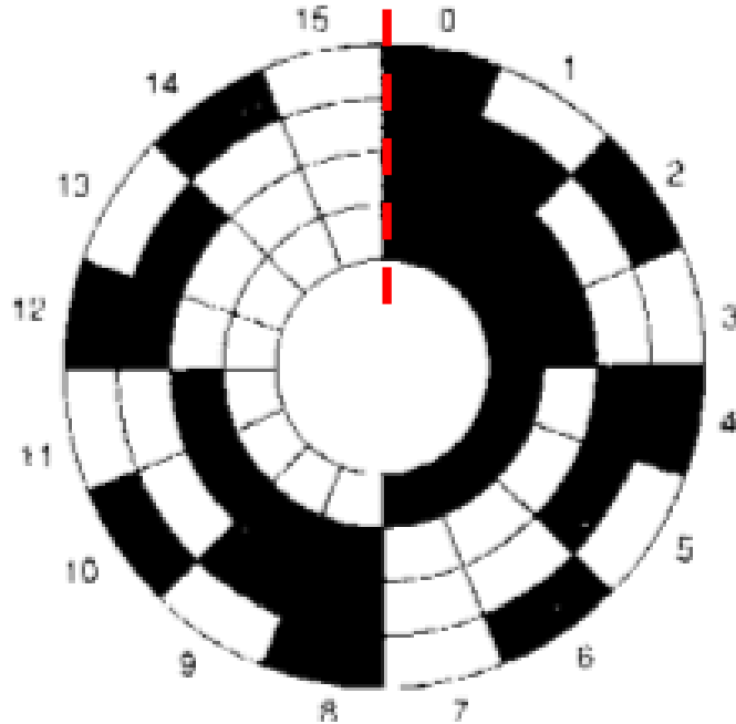
Pure binary code
